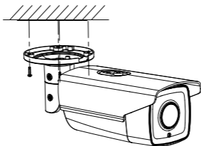
Figure 2-2 Install the Camera
